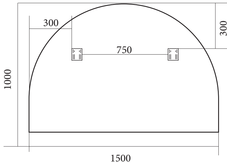
MIRO-FA1500
