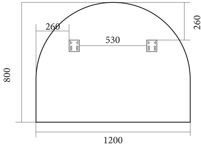
MIRO-FA1200
